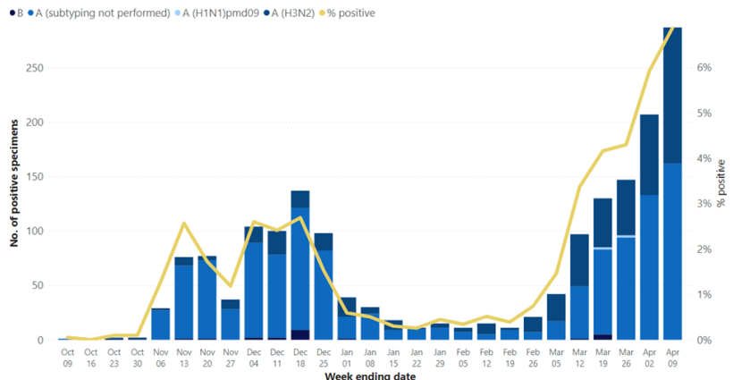
Number and percent of specimens testing positive (by KI+PLK) for influenza by subtype
