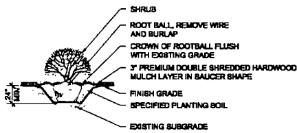
3 SHRUB PLANTING SECTION NOT TO SCALE
