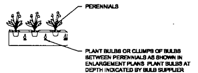
5 BULB INSTALLATION DETAIL NOT TO SCALE
