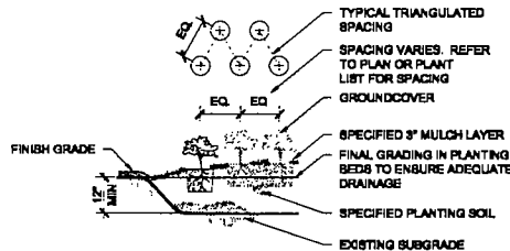
4 PERENNIAL PLANTING SECTION NOT TO SCALE
